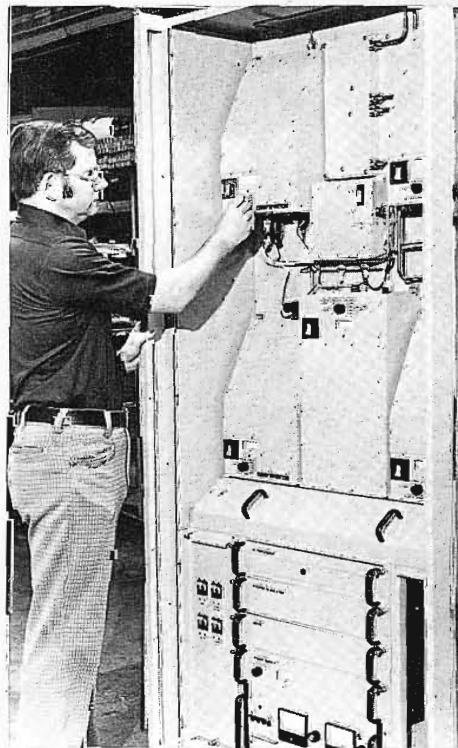
RCA technician checks one of the all-solid-state power amplifiers in the new TTG television transmitter. Four of the amplifiers produce 1600 watts of visual power drive capability, with no tubes and no tuning required.
