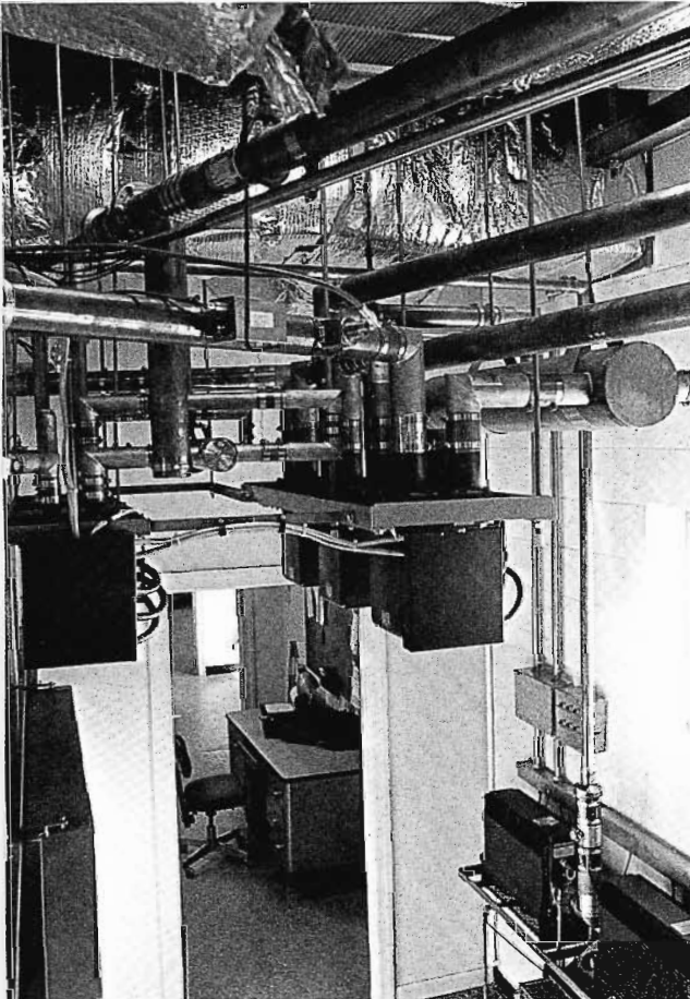
TT-50FL combining and switching—overhead.
