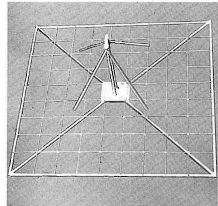
BFJ FM Panel Antenna has produced excellent results for WRAL-FM.
